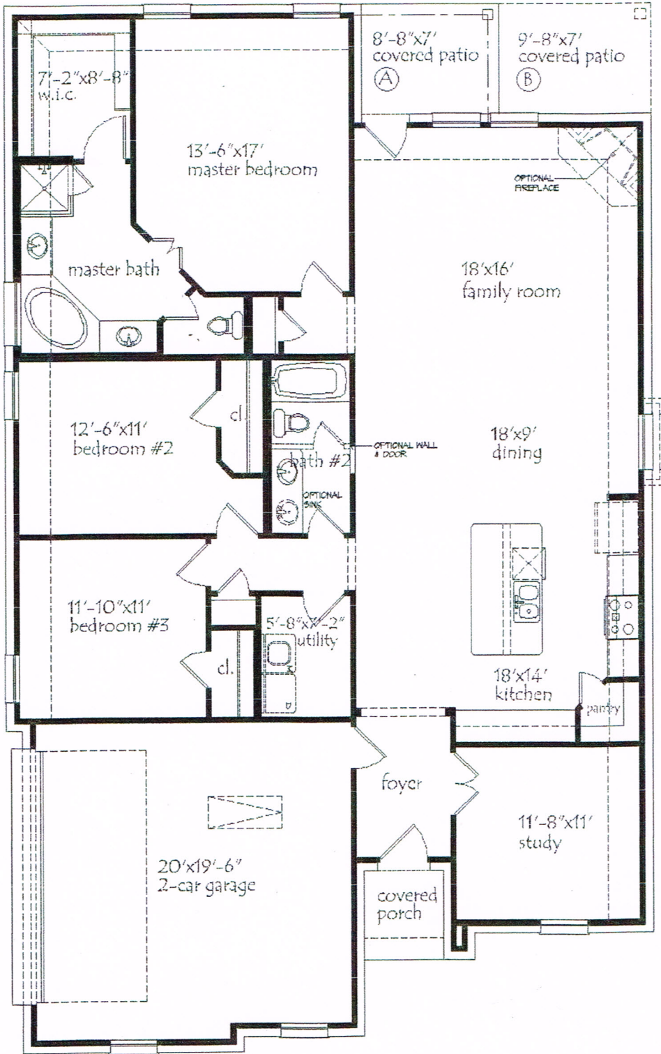
FLOOR PLAN
