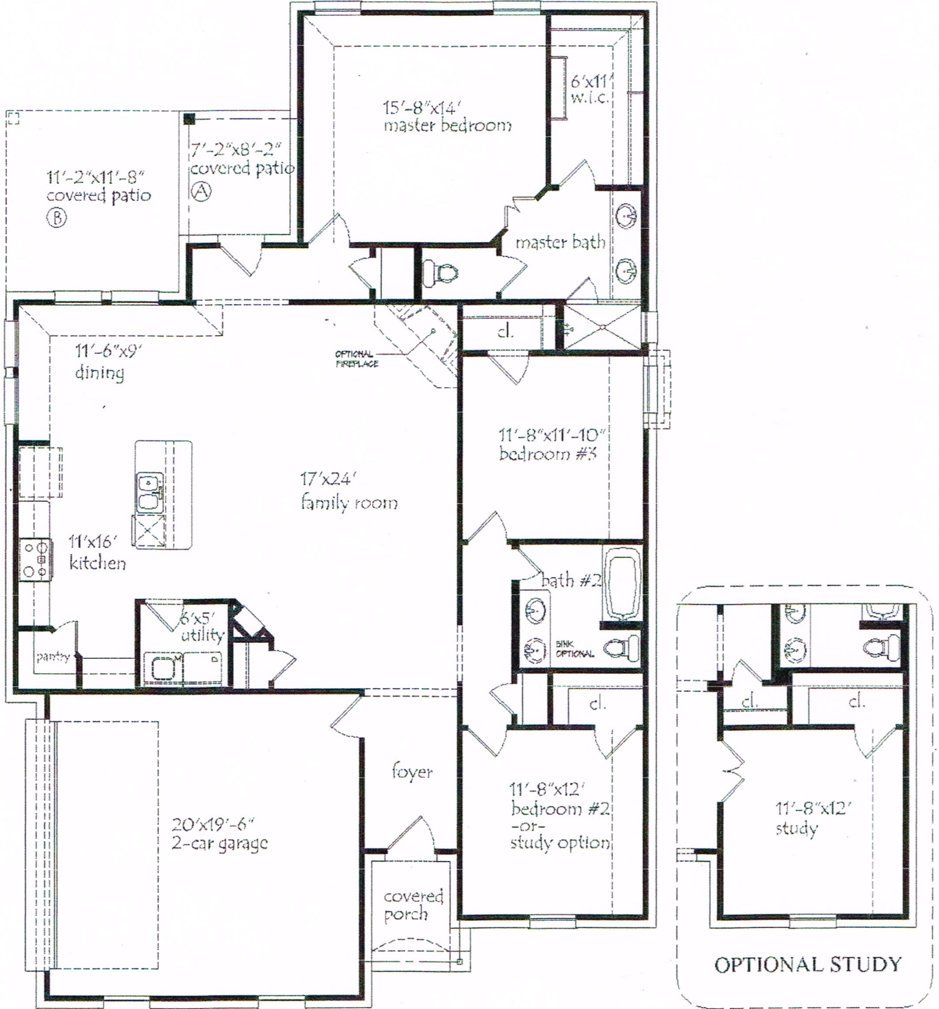
FLOOR PLAN
